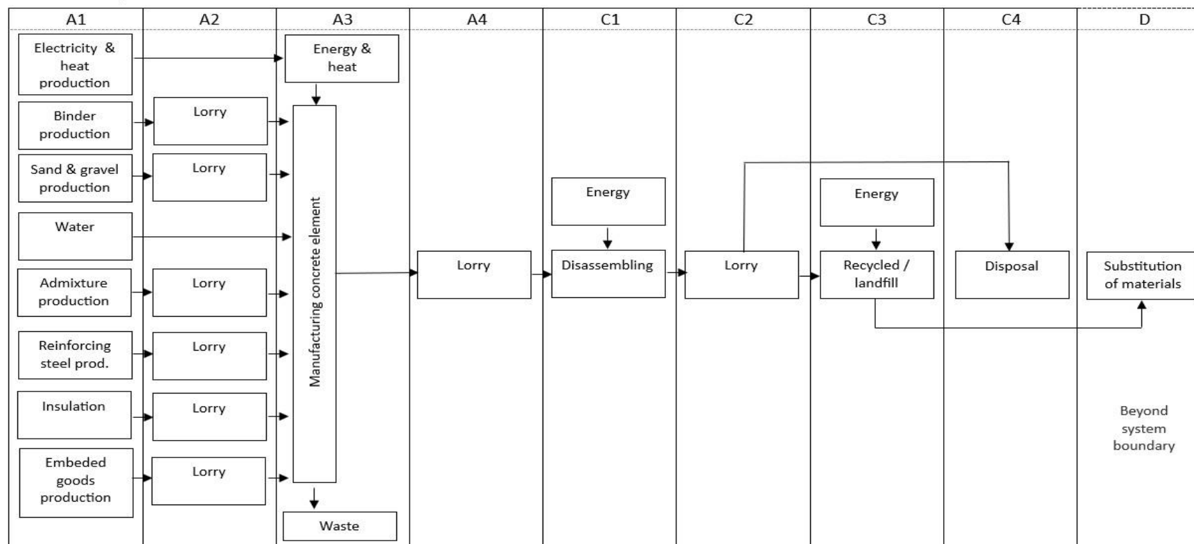
Flowchart over production
